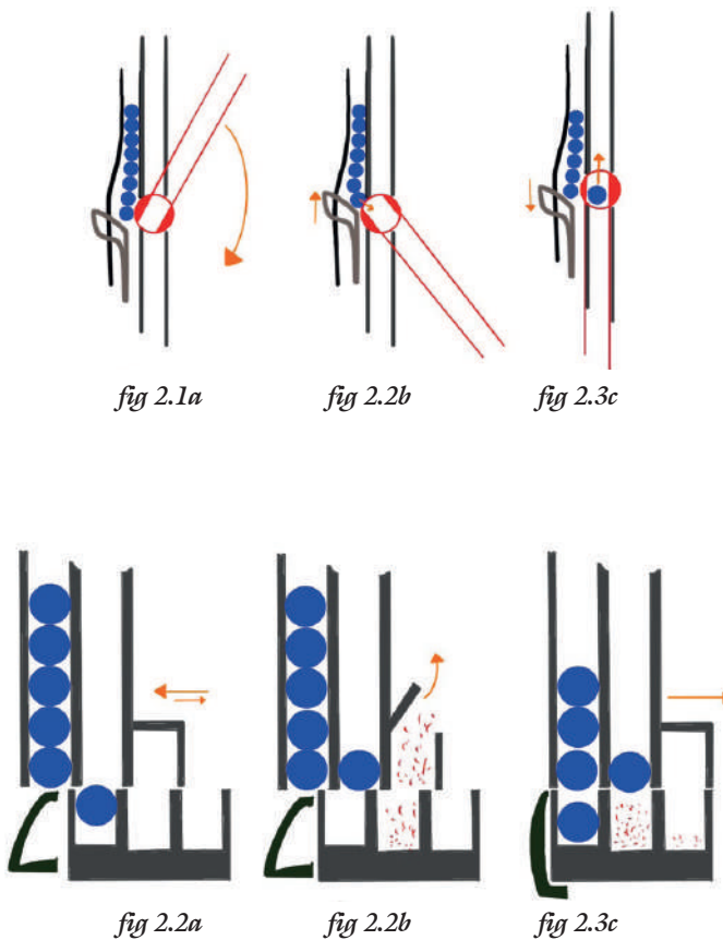
Figure 2. Basic feeding system
